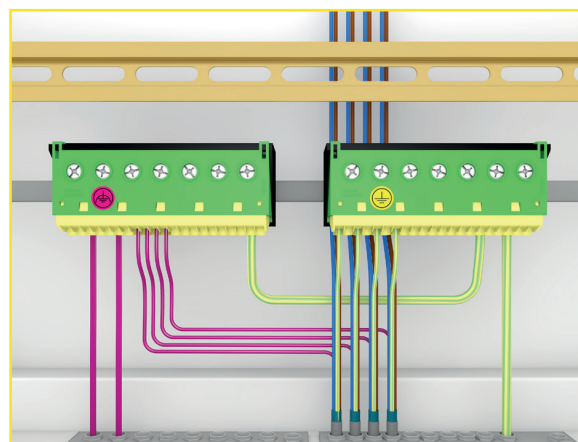
Mark functional potential bonding for clarification. Connect main earthing bar to PE as usual, connect busbar FPA and busbar PE with \geq 4 mm 2 cross-section.
