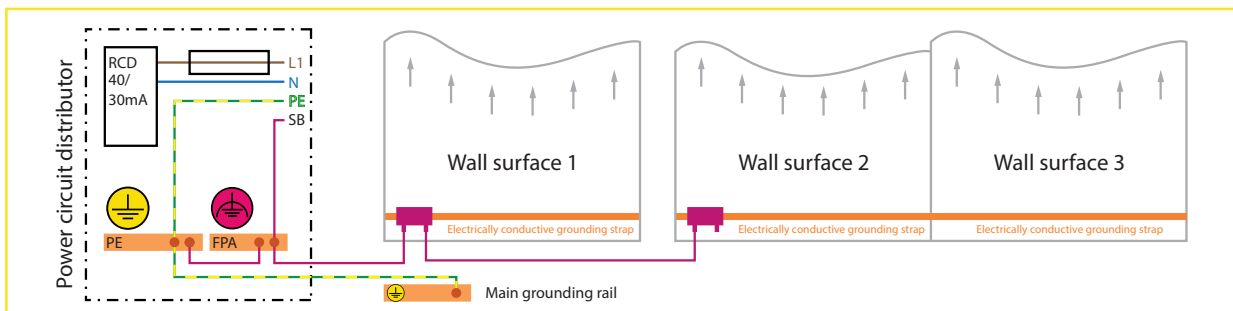
Connection diagram functional potential bonding - shielding surfaces.
